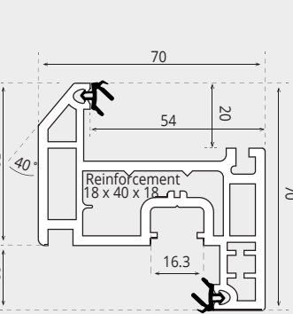
TILT/TURN SASH 70mm
