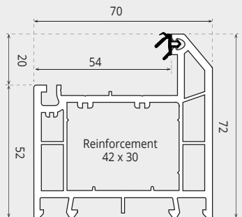
LARGE OUTERFRAME 72mm (3 CHAMBER)
