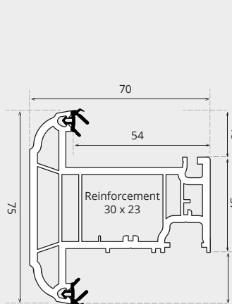
'T' SASH 75mm (5 CHAMBER)
