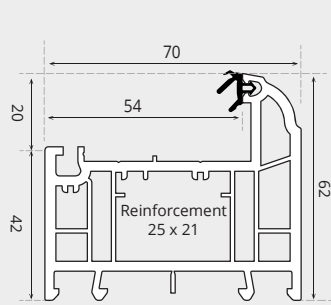
INTERMEDIATE OUTERFRAME 62mm (5 CHAMBERS)
