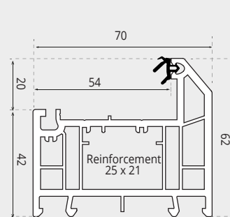
INTERMEDIATE OUTERFRAME 62mm (5 CHAMBER)
