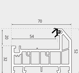
SLIM OUTERFRAME 52mm (6 CHAMBER)
