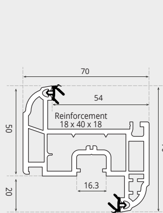
TILT/TURN SASH 70mm
