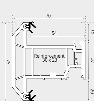
CASEMENT 'T' SASH 75mm (5 CHAMBER)
